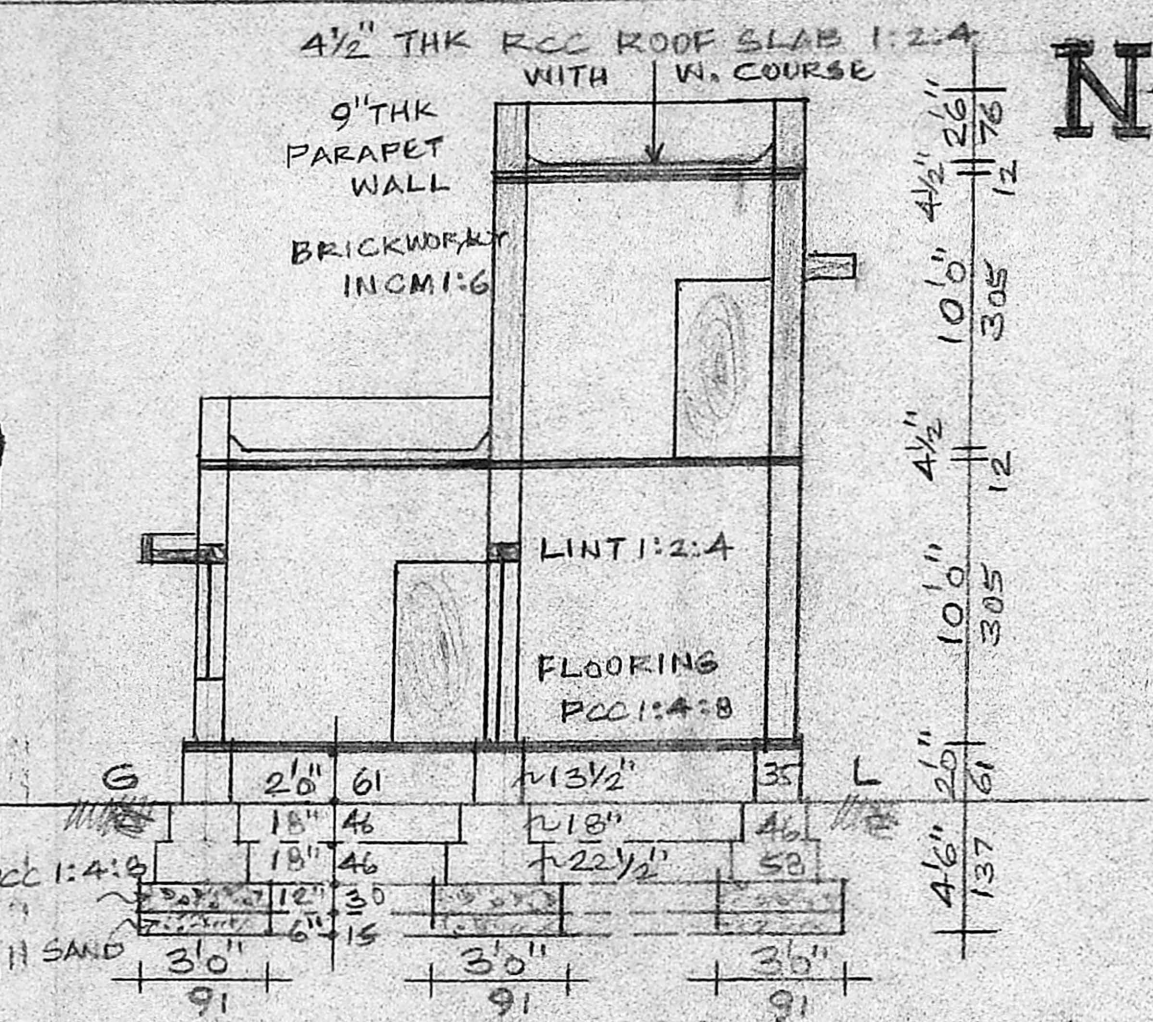
SECTION "AB"
